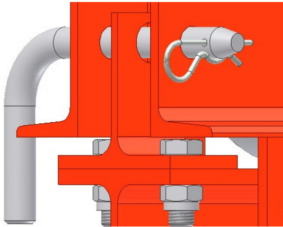
13.10.89 Pin | Cotter Pin
